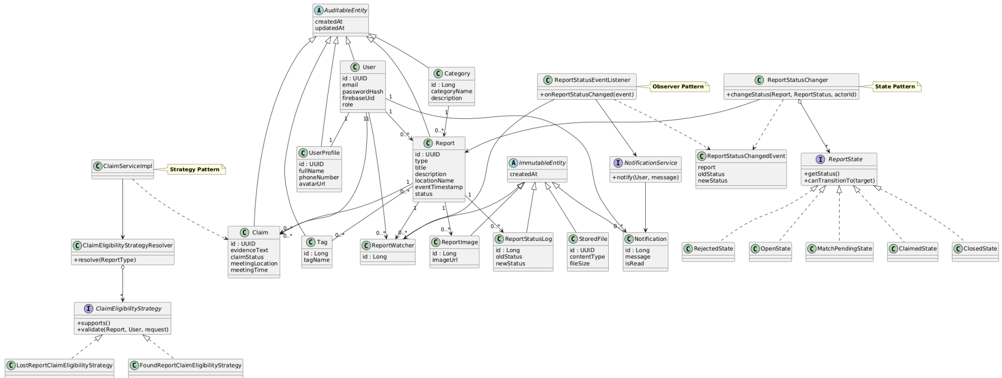
Class Diagram
